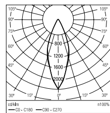
Wide Flood 35°
