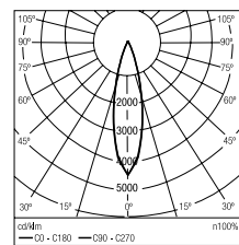
Flood 25°
