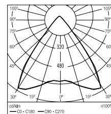
Extensive 75°
