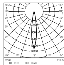
Spot 15°
